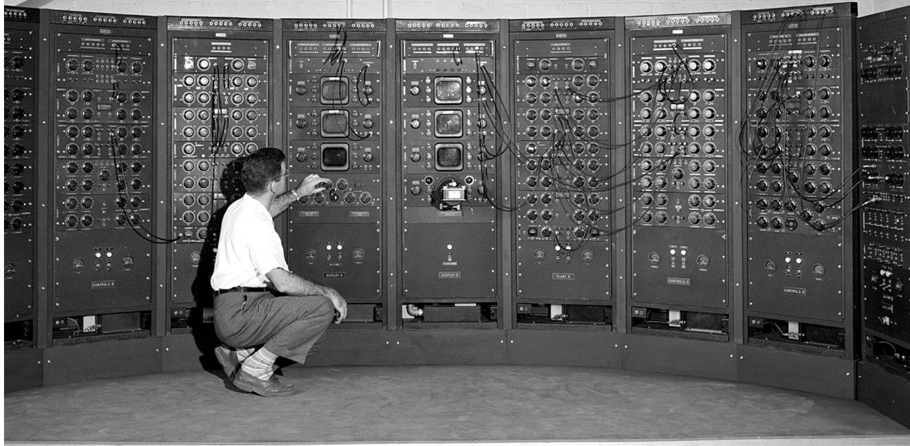
Analog computing machine at the Lewis Flight Propulsion Laboratory circa 1949.
